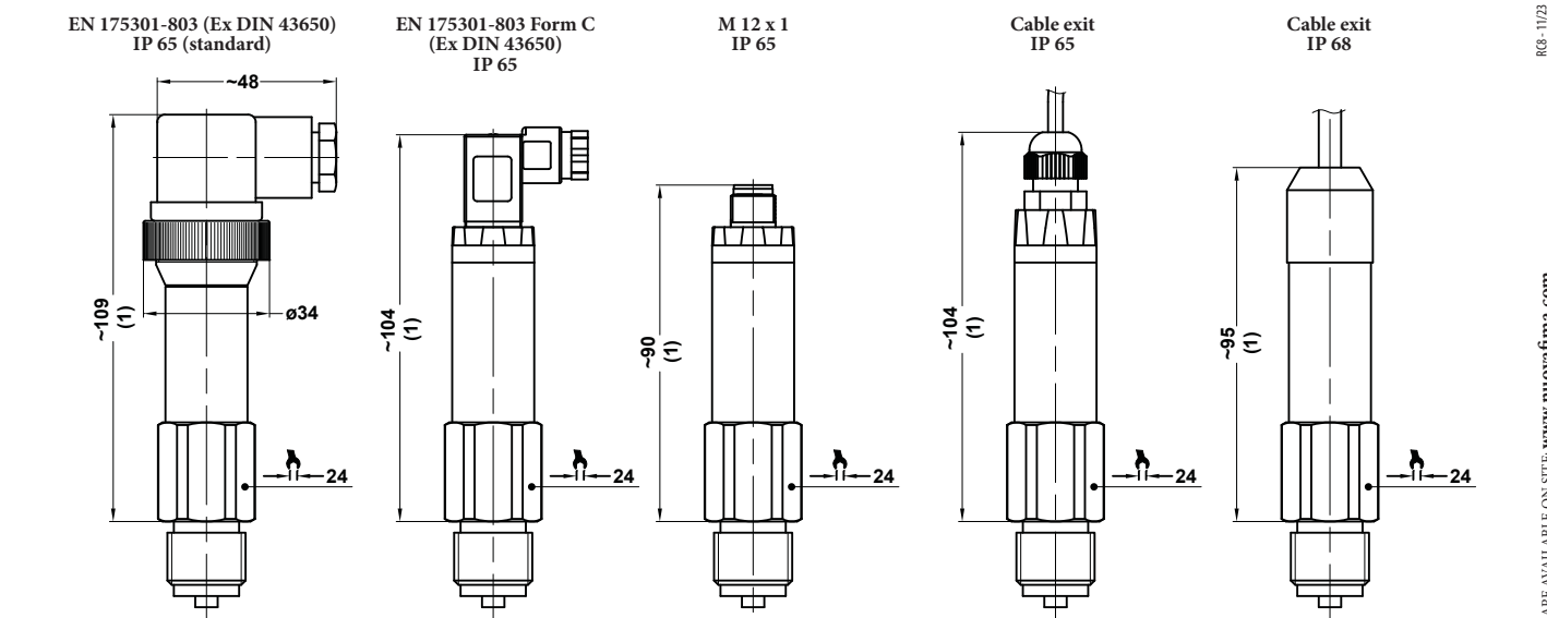
Dimensions: mm; (1) for pressures ≥ 160 bar add 5 mm
