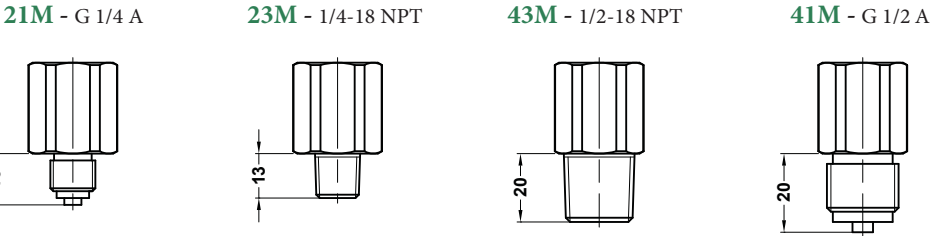
Dimensions: mm; (1) for pressures ≥ 160 bar add 5 mm
